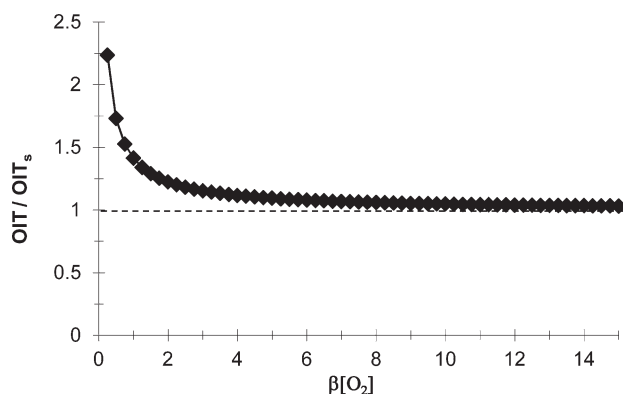
Figure B2. Oxidation induction time versus oxygen partial pressure.
